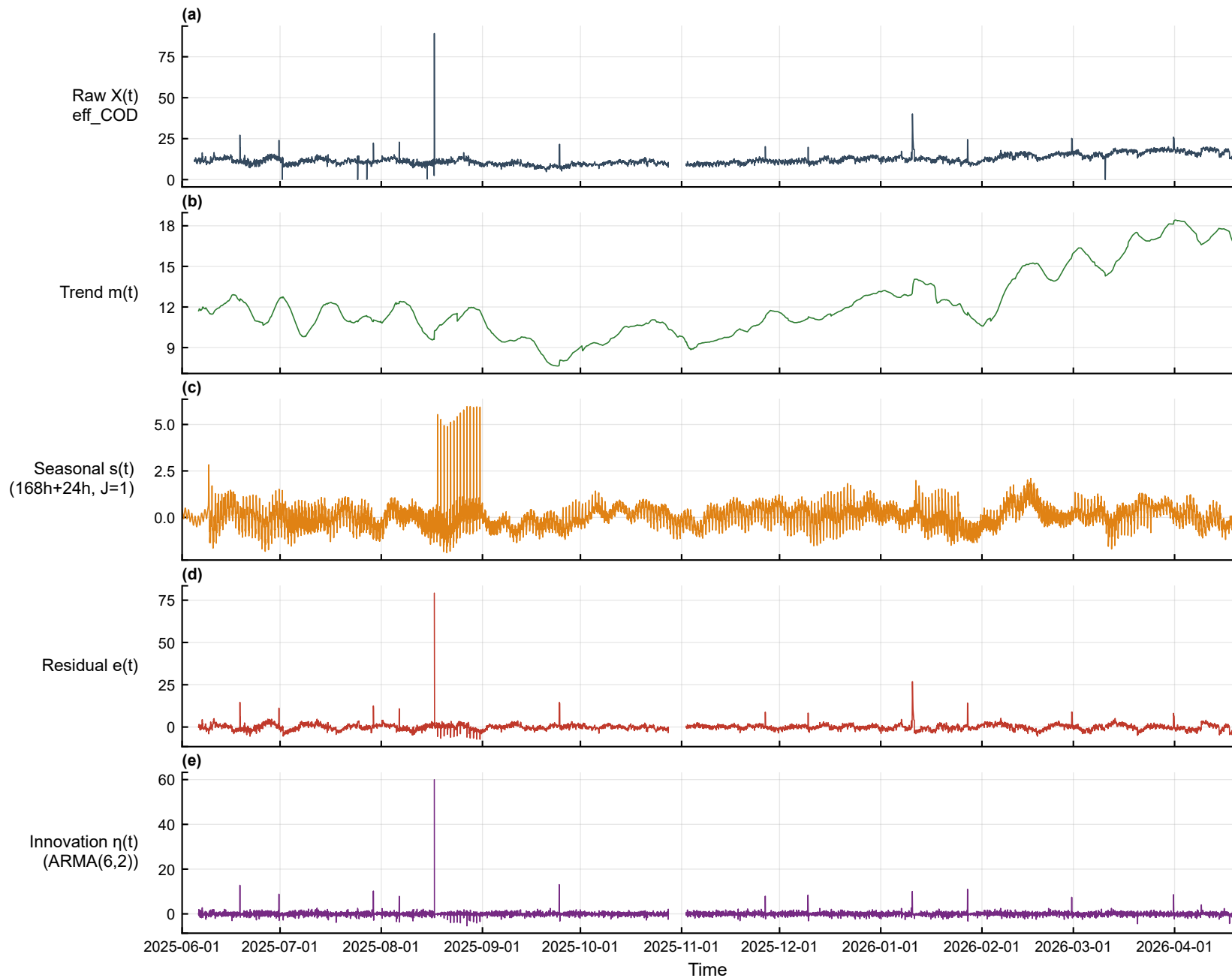
Multi-scale decomposition — eff_COD (effluent, hour) [2025-06-01~2026-04-19]
